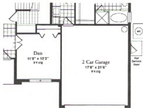
Optional Den with 2 Car Garage
